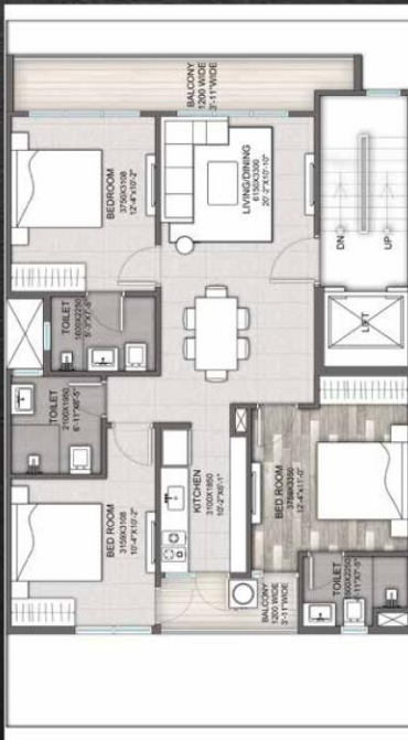
1 ST TO 4 TH FLOOR PLAN
